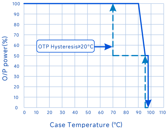
Output Power Vs. Case Temperature
